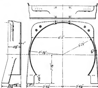
Figs. 213-215. Details of Hip Joint Casing. Atlantic (4—4—2) Locomotive. Pennsylvania Railroad. (193)
